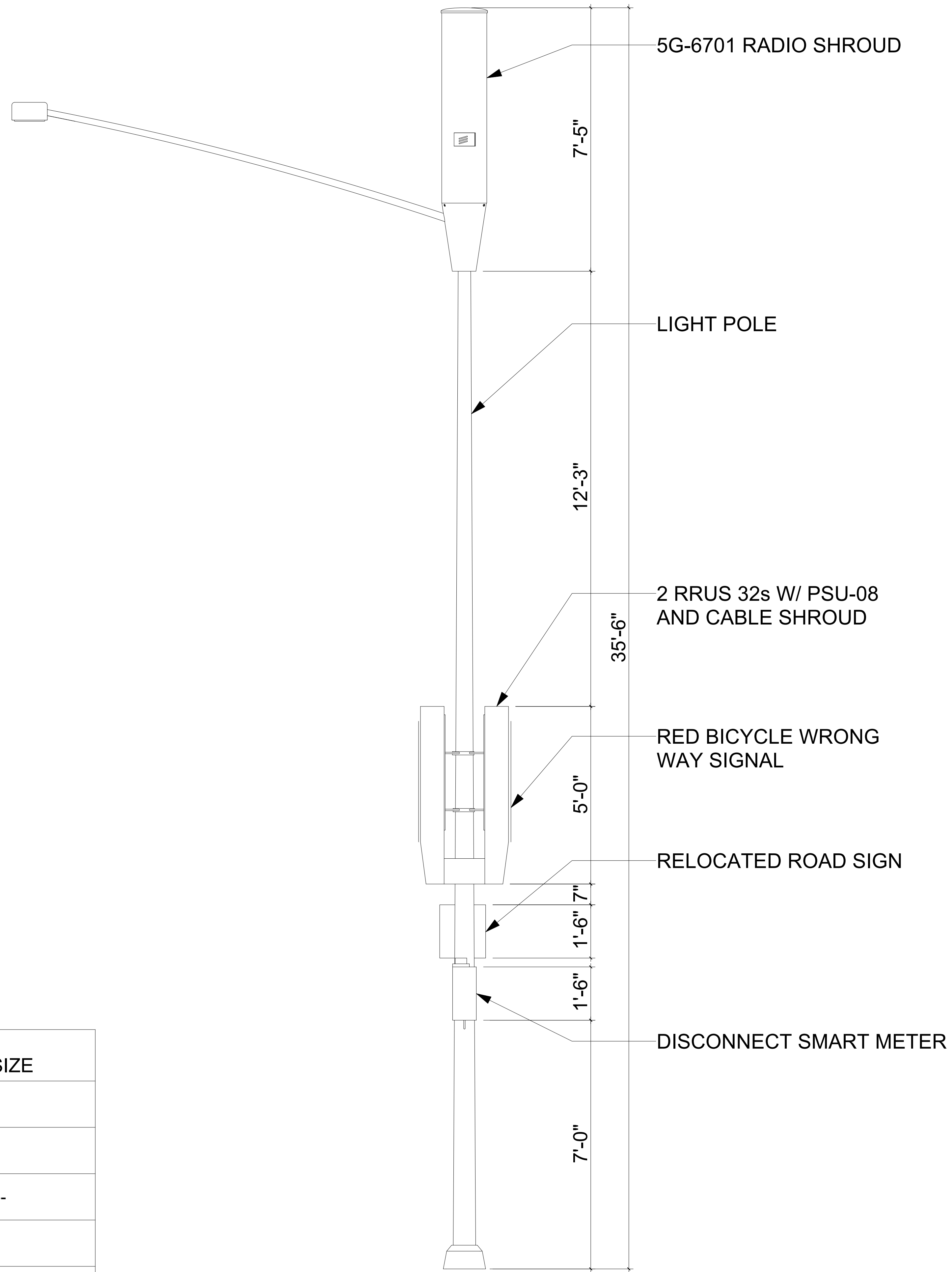
5G-6701 RADIO CAGE LIGHT POLE
