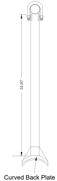
PLAN VIEW
